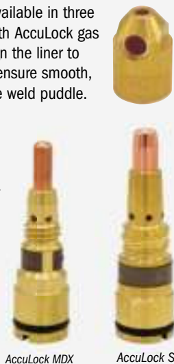
AccuLock MDX
